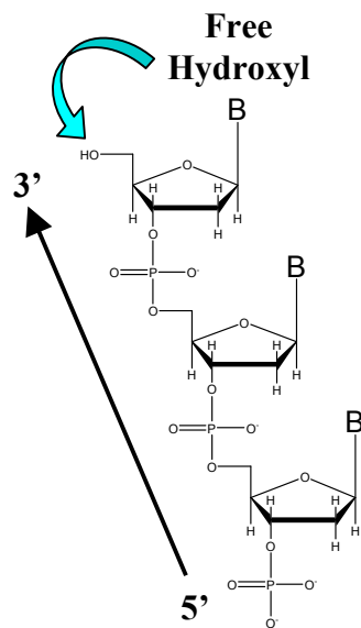
Fig. 2. A schematic view of a short stretch of single stranded DNA showing the sugar-phosphate backbone and the 5' to 3' orientation of the strand.
