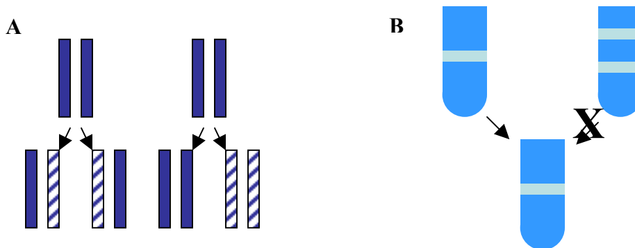
Fig. 1. A. Semiconservative (left) and conservative (right) DNA replication models. B. The DNA sedimentation results obtained by Meselson and Stahl (1958). The two tubes on top represent the expected results for semiconservative (left) and conservative (right) DNA replication. The lower tube is the experimental observation.
