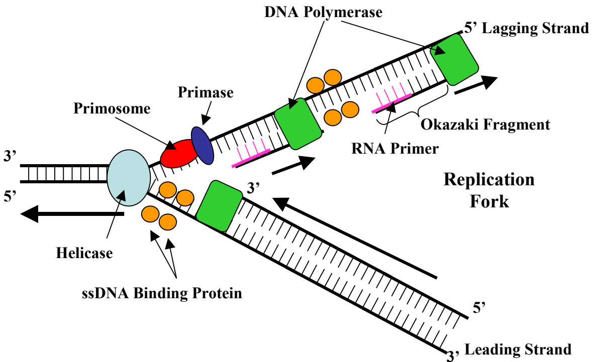
Fig. 4. Anatomy and organization of the DNA replication fork.
