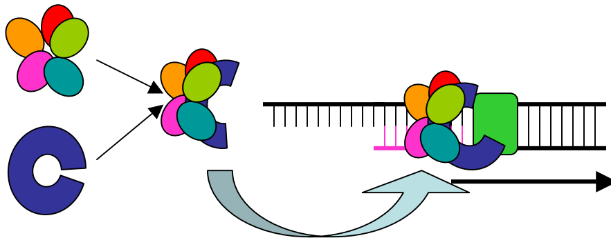
Fig. 5. Schematic representation of a sliding clamp-clamp loader complex delivering the clamp to a DNA molecule in the process of replication. The five-subunit clamp loader complexes with the clamp and opens it up. The clamp-clamp loader complex then binds to the DNA polymerase. The clamp closes and the polymerase speeds off to carry out replication.
