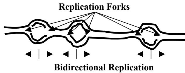
Fig. 3. A representation of DNA replication proceeding from several different points of origin.
